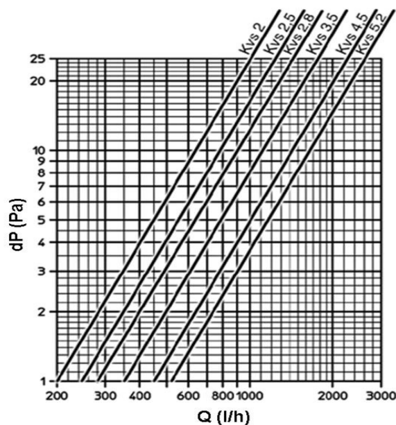
Pressure drop
